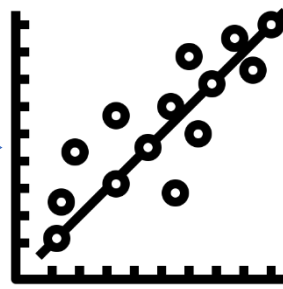
Regression
